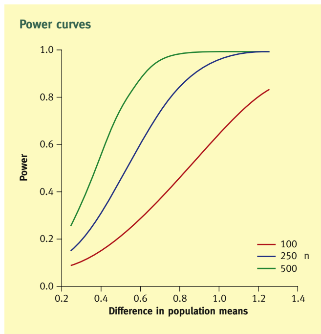
Figure 2 Power curves demonstrating the power for various sample sizes to be able to detect a range of differences between two groups (for control population mean of 2.6, a standard deviation of 3 and \alpha (type 1 error probability) = 0.05). Plotted using the free software package 'Power and Sample Size Calculation' by WD Dupont and WD Plummer. 8
